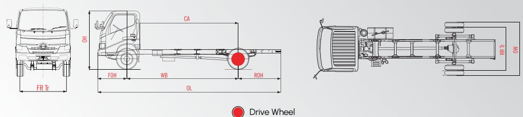
Dimensi Hino 300 Series | 136 MDLR
